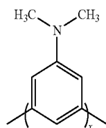
Poly(1,3-(5-dimethylamino)phenylene), 24
